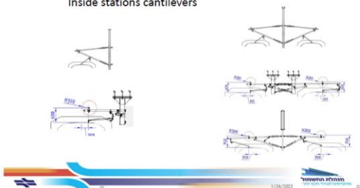
Inside stations cantilevers
