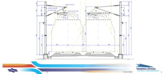
STRAIGHT TRACK
